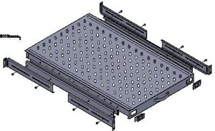
Explode View
