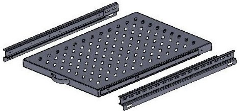
Explode View
