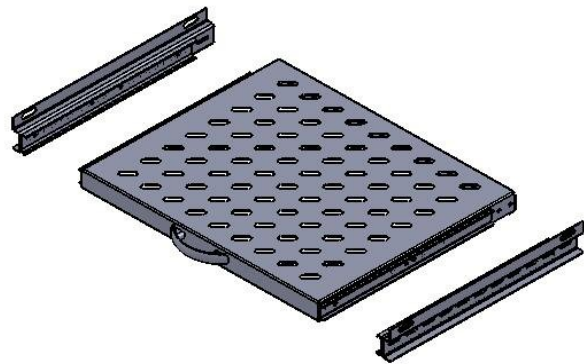
Explode View
