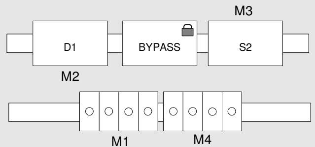
Implantation coffret 2*12 Modules UPS 20/30/40/60 KVA
